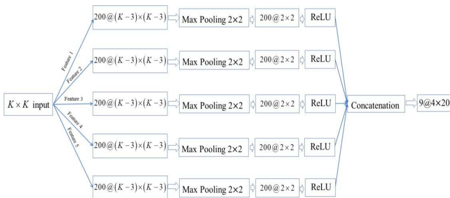
Figure 9. The network architecture with different inputs of different neighborhood sizes.
