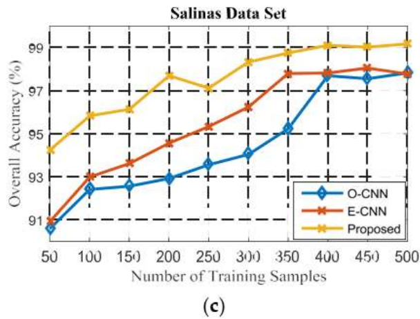
Figure 8. The effects of training samples on accuracies of three data sets: (a) Indian Pines; (b) University of Pavia; (c) Salinas.
